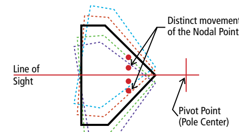
Non-Aligned at 0 mm Offset
